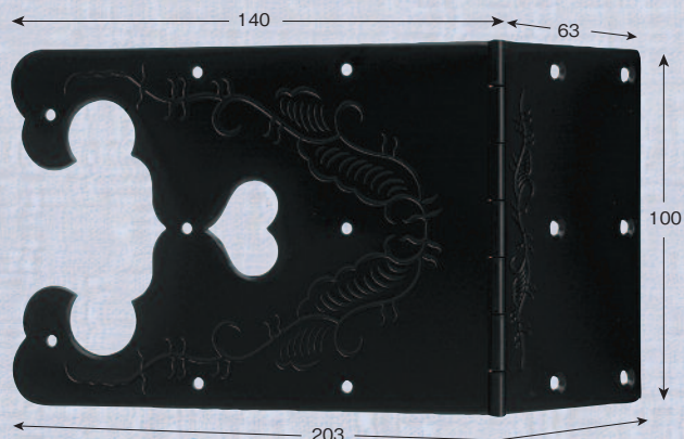
伊達飾 No.340 平丁双
