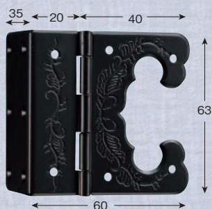
伊達飾 No.350 曲丁双
